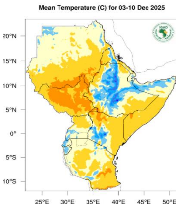
Figure 4 – Mean temperature forecast for 03 -10 Dec 2025 (Source: ICPAC).
