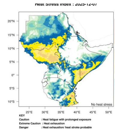
Figure 6 - Heat Stress Index: 2025-11-23 03 -10 Dec 2025 (Source: ICPAC).
