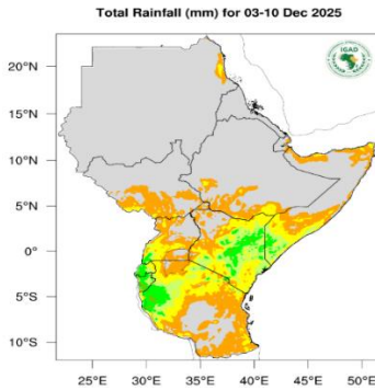
Figure 1 - Total rainfall forecast 03 -10 Dec 2025 (Source: ICPAC).
