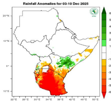
Figure 2 - Rainfall anomalies forecast 03 -10 Dec 2025 (Source: ICPAC).
