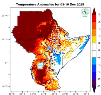
Figure 5 - Temperature Anomalies for 03 -10 Dec 2025 (Source: ICPAC).
