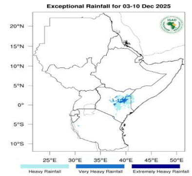
Figure 3 - Exceptional Rainfall forecast 03 -10 Dec 2025 (Source: ICPAC)
